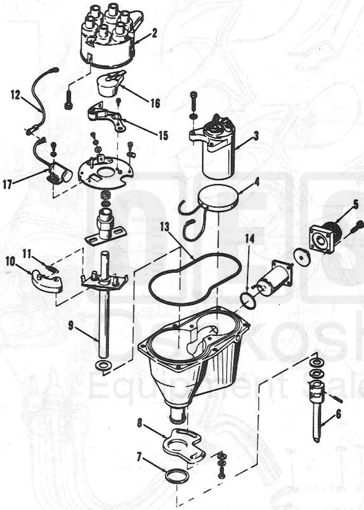
Figure 39: Ignitor Assembly
